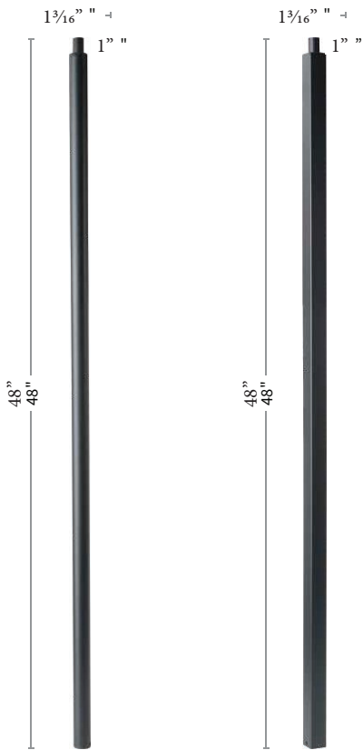
9501HN-SB-48 Round Hollow Newel Post Satin Black
